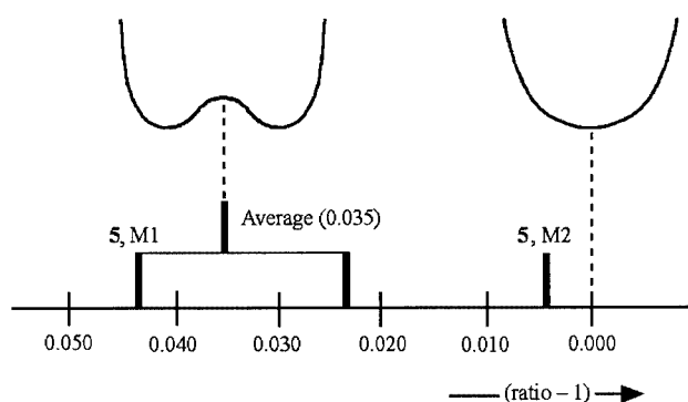
Figure 11. View of the situation present in 2-aminotroponimines regarding the exocyclic C–N bonds
