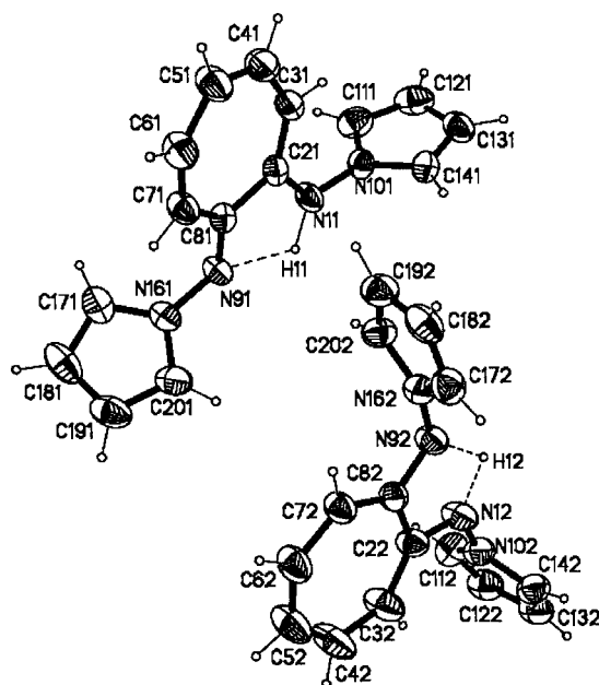
Figure 5. X-ray asymmetric unit of N -(pyrrol-1-yl)-2-(pyrrol-1-yl-amino)troponimine ( 5 )
