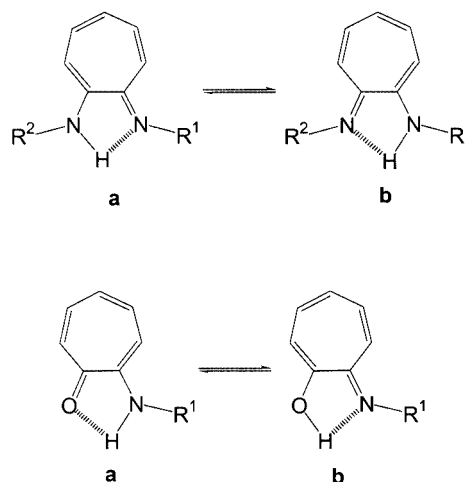
Scheme 1. Tautomeric forms for 2-aminotroponimines and 2-aminotropones
