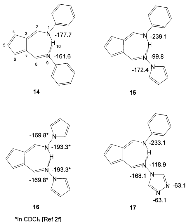
Figure 10. ^{15}\text{N} CPMAS NMR spectroscopic data [2d,2e,14] for 6-aminofulvene-1-aldehydes 14–17
