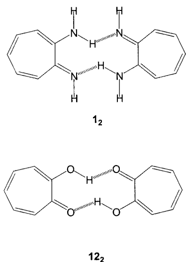
Figure 9. 2-Aminotroponimine and tropolone dimers
