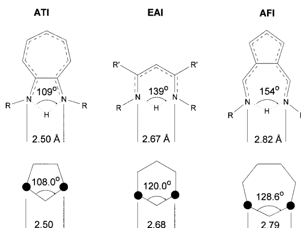
Figure 12. Experimental distances and angles involved in hydrogen bonding for 2-aminotroponimines ( ATI ), \beta -enaminoimines ( EAI ) and 6-aminofulvene-1-aldehydes ( AFI )
