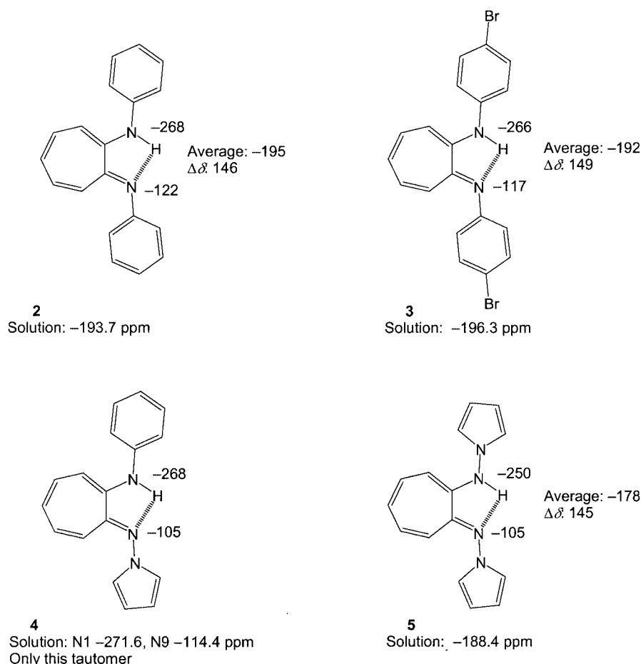
Figure 6. ^{15}\text{N} CPMAS NMR spectroscopic data for 2-aminotroponimines 2–5
