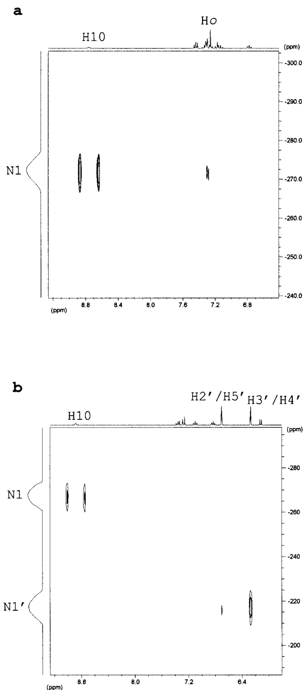
Figure 7. gs-HMBC correlation spectra: a) compound 7 in \text{CDCl}_3 ; b) compound 10 in \text{CDCl}_3
