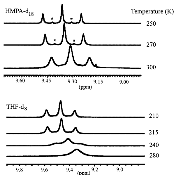
Figure 8. Variable temperature ^1\text{H} NMR of 2\text{-}^{15}\text{N}_2 (10-H region) in [\text{D}_{18}]\text{HMPA} and [\text{D}_8]\text{THF}
