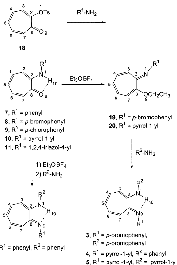
Scheme 2. Outline of the synthetic route used to prepare the compounds
