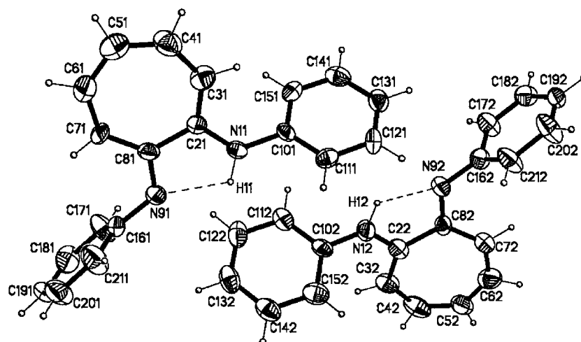
Figure 2. X-ray asymmetric unit of N -phenyl-2-(phenylamino)troponimine ( 2 )
